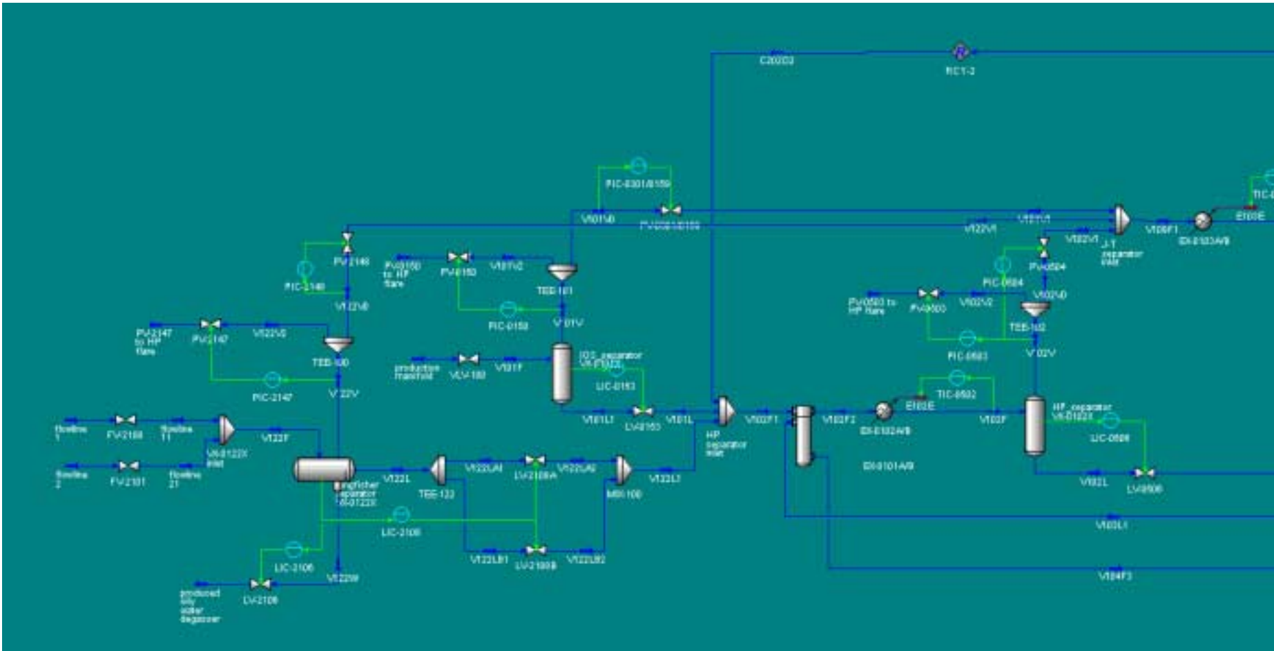
Front-end of oil/gas/water separation process
